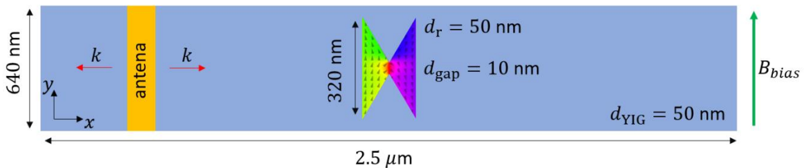
Fig. 1. Schematic picture of the studied system. A YIG waveguide with thickness d_{YIG} = 50 nm. The bias field is applied in the y direction, and SW exciting antenna is shifted from the center. The bowtie-shaped resonator is placed d_{gap} = 10 nm above the waveguide, it is 320 nm wide, and d_r = 50 nm thick. The resonator is non-collinearly magnetized with magnetization in the left trapezoid pointing in the +y direction, and -y in the right. Between the trapezoids a formation of a domain wall is visible.
